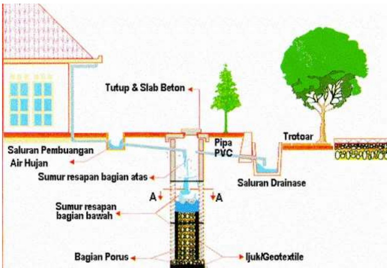
Gambar 6.2. Diagram Sumur Resapan
